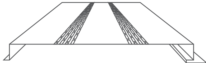
SINGLE OR DOUBLE VENTED (NET FREE AREA/12" IS 2.65 SQ IN/VENT)
